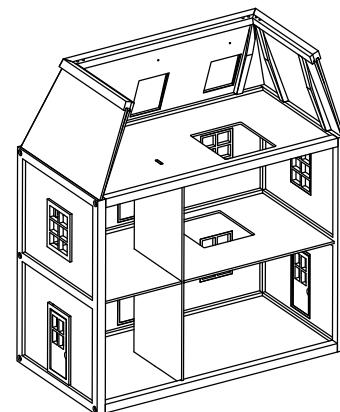
Assembled View
